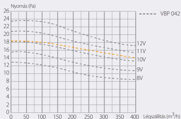
Jelleggörbék
